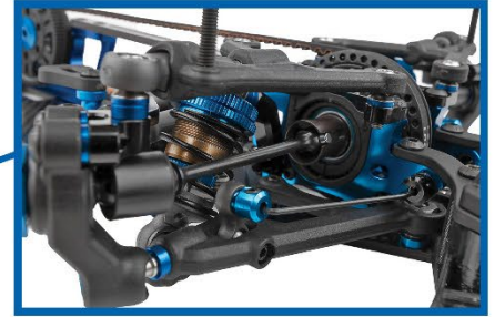
Long-Arm Pivot Ball Suspension Geometry
